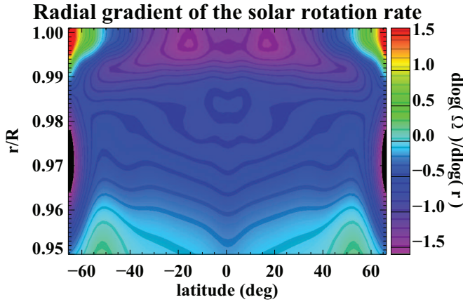
Figure 3. Variations of the rotational gradient, d \log \Omega / d \log r , in the leptocline a) with the depth below the solar surface at three latitudes, and b) with latitude at three depths (shown in the figure); c) latitude-radius diagram of the rotational gradient in the NSSL and leptocline.
