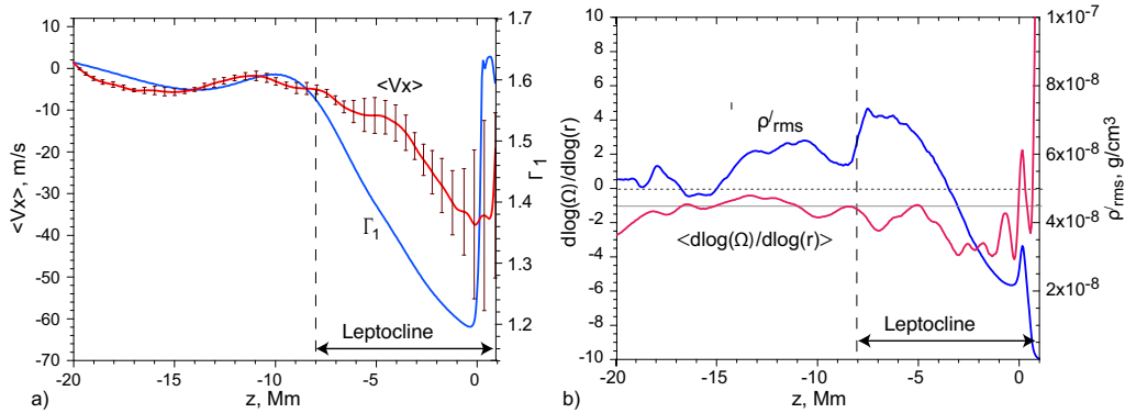
Figure 6. Mean radial profiles of a) deviations of the azimuthal flow speed from the imposed rotation rate at 30 degrees latitude (red curve) and the adiabatic index, \Gamma_1 (blue curve); b) the radial gradient of the rotation rate, defined as \partial \log \Omega / \partial \log r (red curve), and the RMS density perturbations, \rho'_{rms} (blue curve). Radial profiles are obtained by averaging a 24-hour series of 3D simulation data horizontally over the simulation domain and in time. The vertical bars show 1\sigma flow velocity deviations from the mean values. The data in this figure are adapted from (Kitiashvili et al. 2023).
