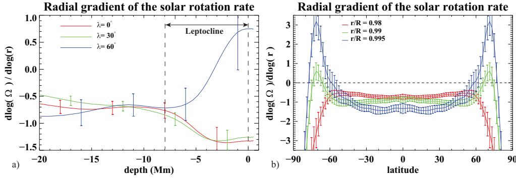
Figure 2. The radial gradient of the mean rotation rate, averaged over all SoHO/MDI and SDO/HMI measurements in 1996-2024, as a function of depth in the near-surface shear layer at 0^\circ , 30^\circ , and 60^\circ latitudes.
