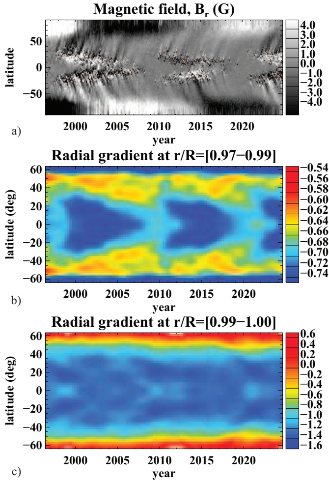
Figure 4. a) The magnetic time-latitude (“butterfly”) diagram for the radial component of the line-of-sight magnetic field from the SoHO and SDO data; b-c) the time-latitude diagrams for the rotational gradient, d \log \Omega / d \log r below the leptocline ( r/R = 0.97 - 0.99 ) and in the leptocline ( r/R = 0.99 - 1.00 ) respectively.
