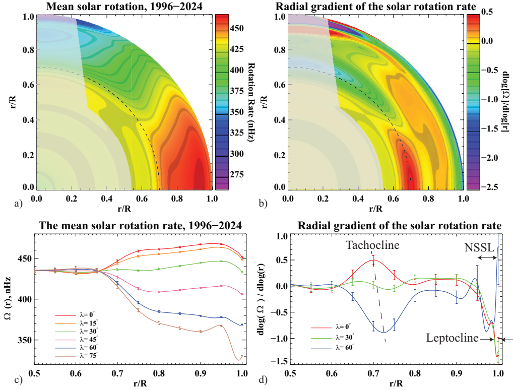
Figure 1. The mean rotation rate, \Omega , and the radial gradient, d \log \Omega / d \log r , averaged over all SoHO/MDI and SDO/HMI measurements in 1996–2024, as a function of radius and latitude. a-b) cross-section views of the rotation rate and the gradient (the shaded region is where the inversion results are uncertain); c) the mean rotation rate at six latitudes indicated in the figure; d) the radial gradient as a function of radius at three latitudes indicated in the figure.
