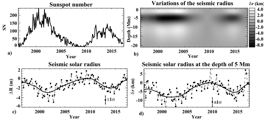
Figure 5. Variations of the seismic radius of subsurface layers during Solar Cycles 23 and 24: a) the sunspot number of these cycles; b) the time-depth diagram of subsurface displacements, \delta r , inferred from f-mode frequencies obtained from the SoHO and SDO data; c) the variations of the Sun’s seismic radius obtained by averaging the displacements of the depth; d) the variations of the seismic radius ( \delta r ) in the leptocline, at a depth of 5 Mm. The data are adapted from Kosovichev and Rozelot (2018).
